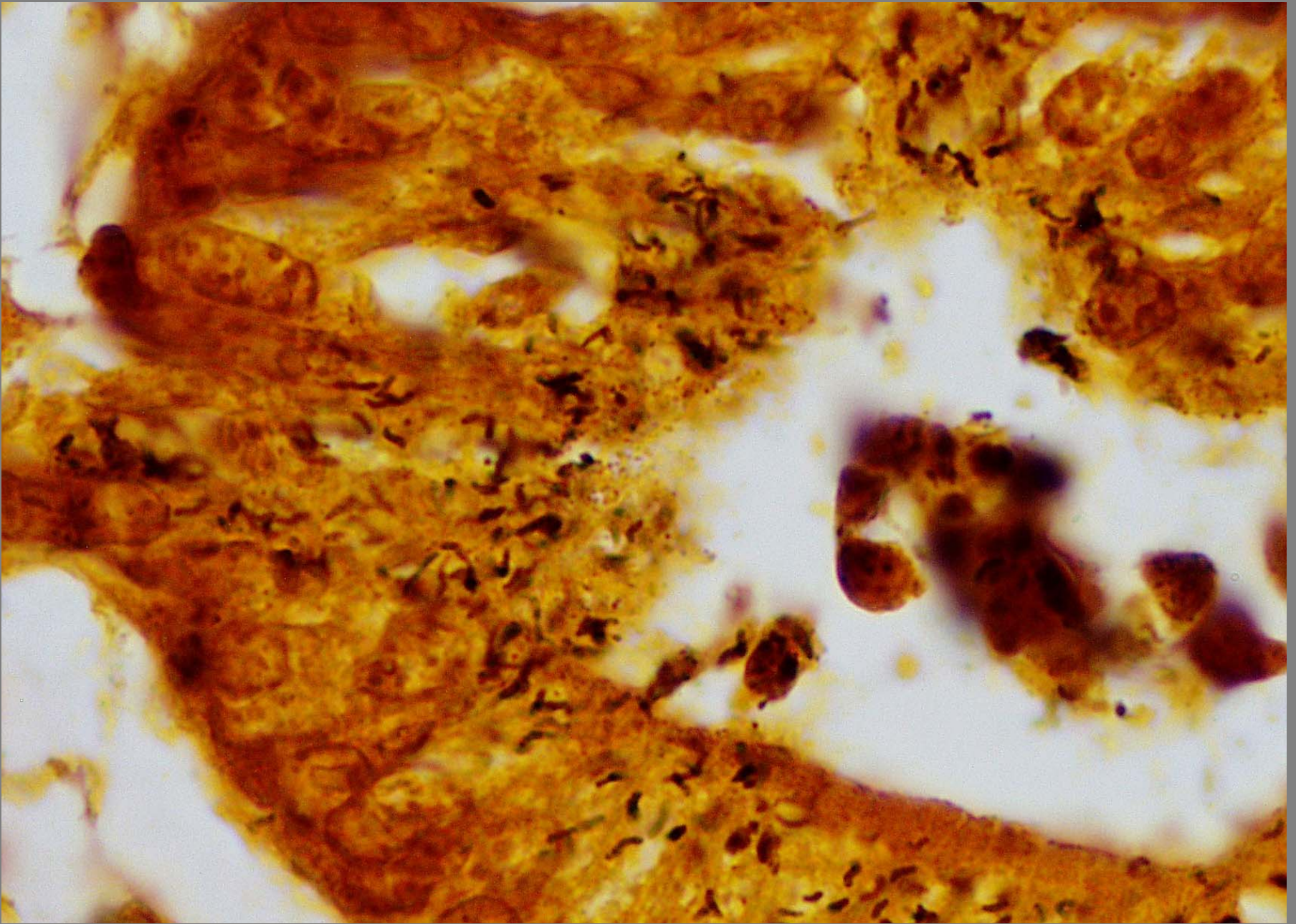
Intestine – proliferative distal ileitis – Lawsonia intracellulare – Whartin Starry stain
